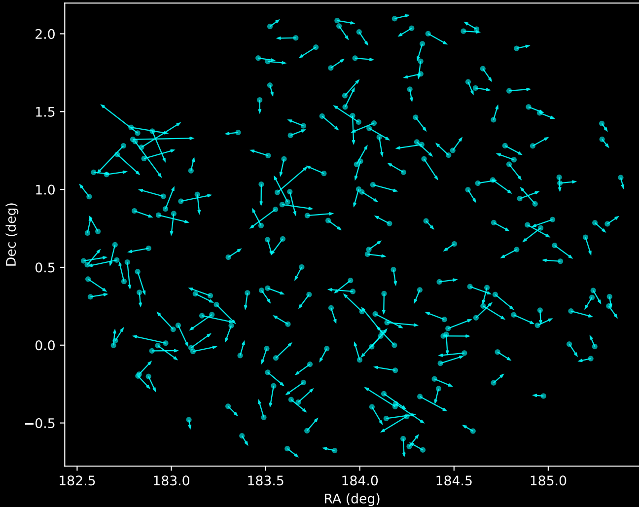
APOGEE DR17 Noise Stream Proper Motion Vectors (n=224)
