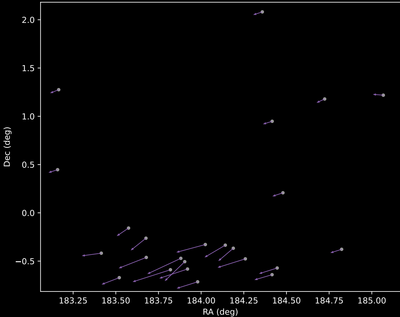
APOGEE DR17 Cluster 8 Proper Motion Vectors (n=24)
