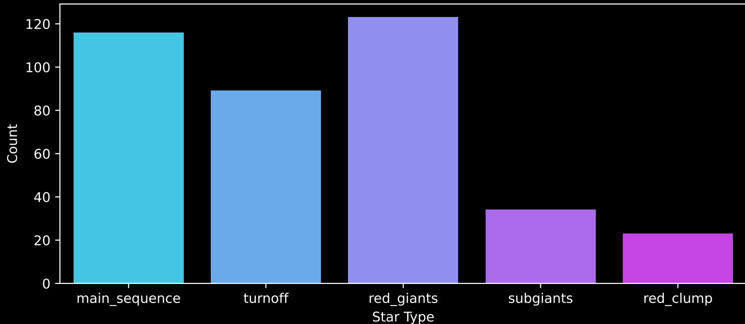
APOGEE DR17 Field: [ORIONOB1AB-B] Count plot of Star Type
