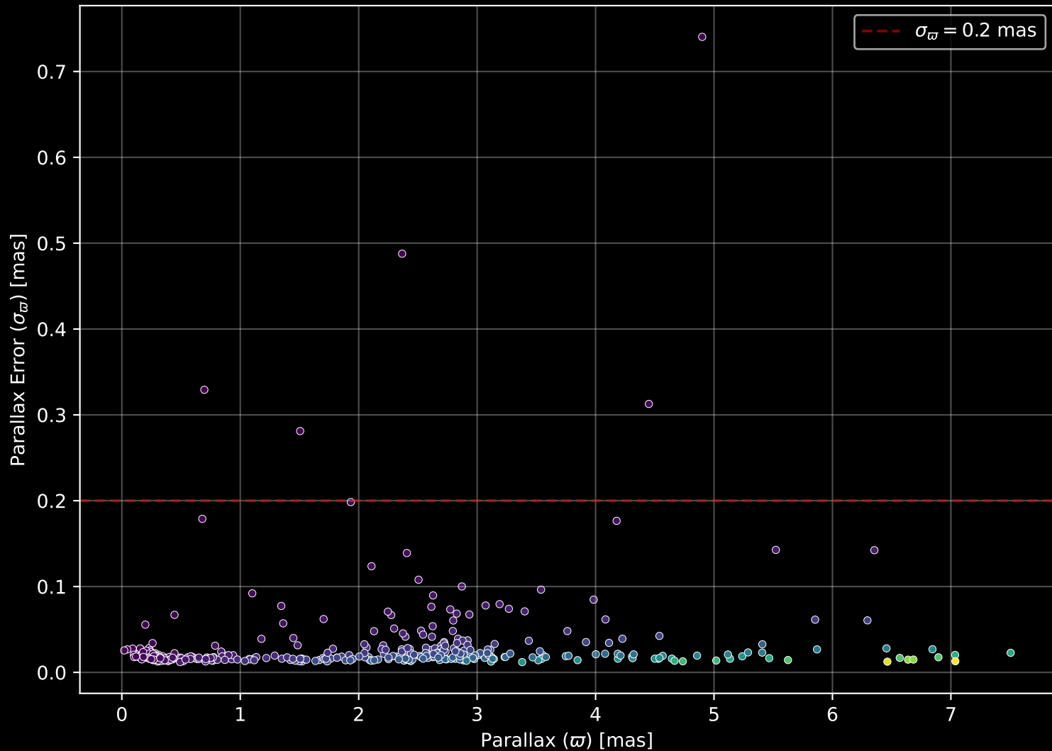
APOGEE DR17 Field: [ORIONOB1AB-B] Parallax Quality (n= 385)
