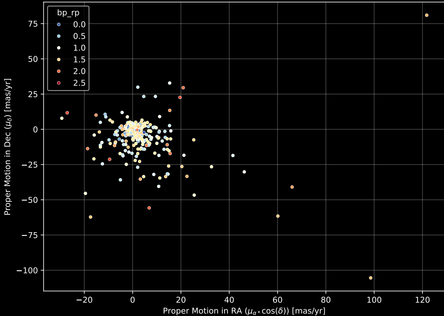
APOGEE DR17 Field: [ORIONOB1AB-B] Proper Motion Diagram (n= 385)
