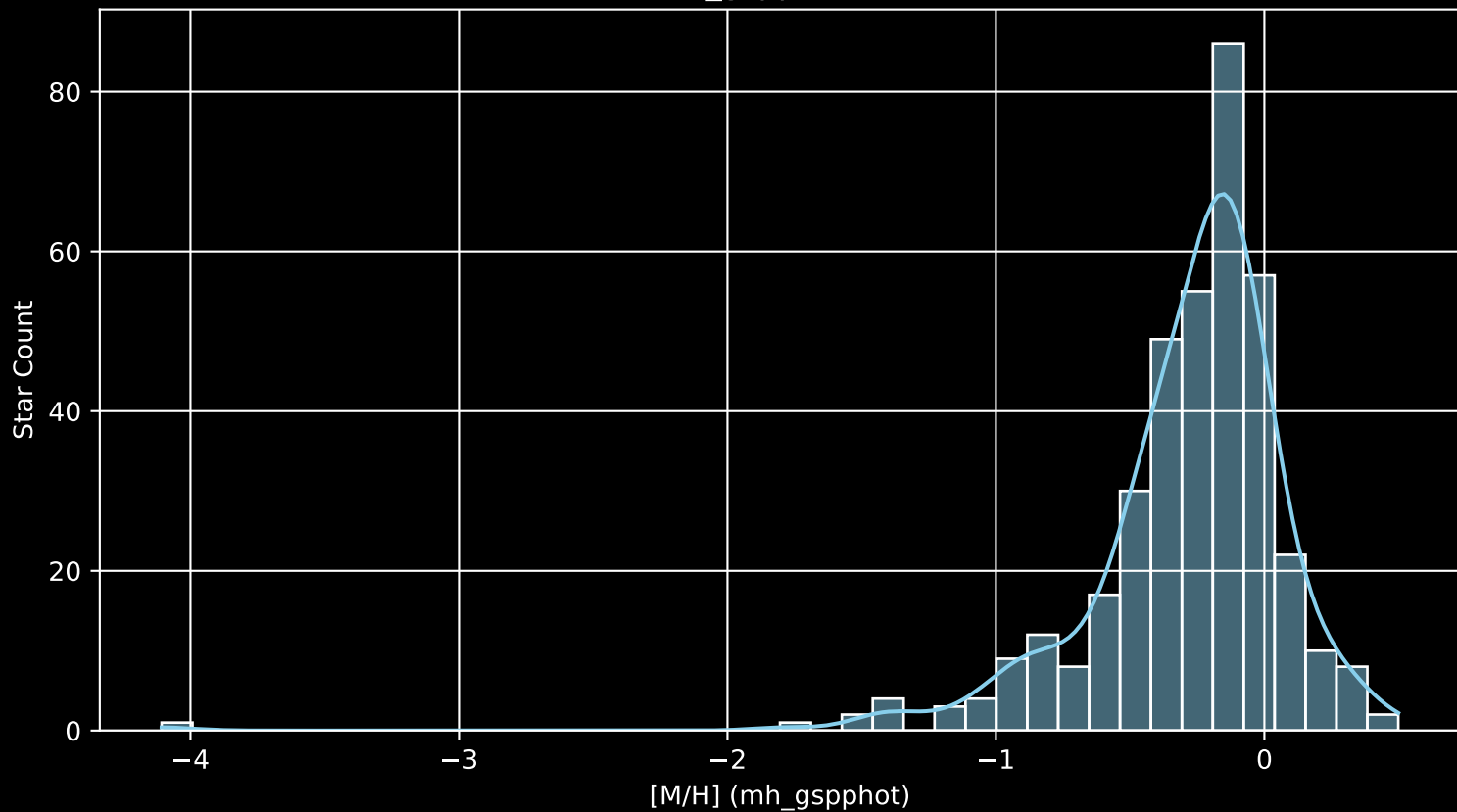
APOGEE DR17 Field: [ORIONOB1AB-B [M/H] (mh_gspphot) (n= 380)
