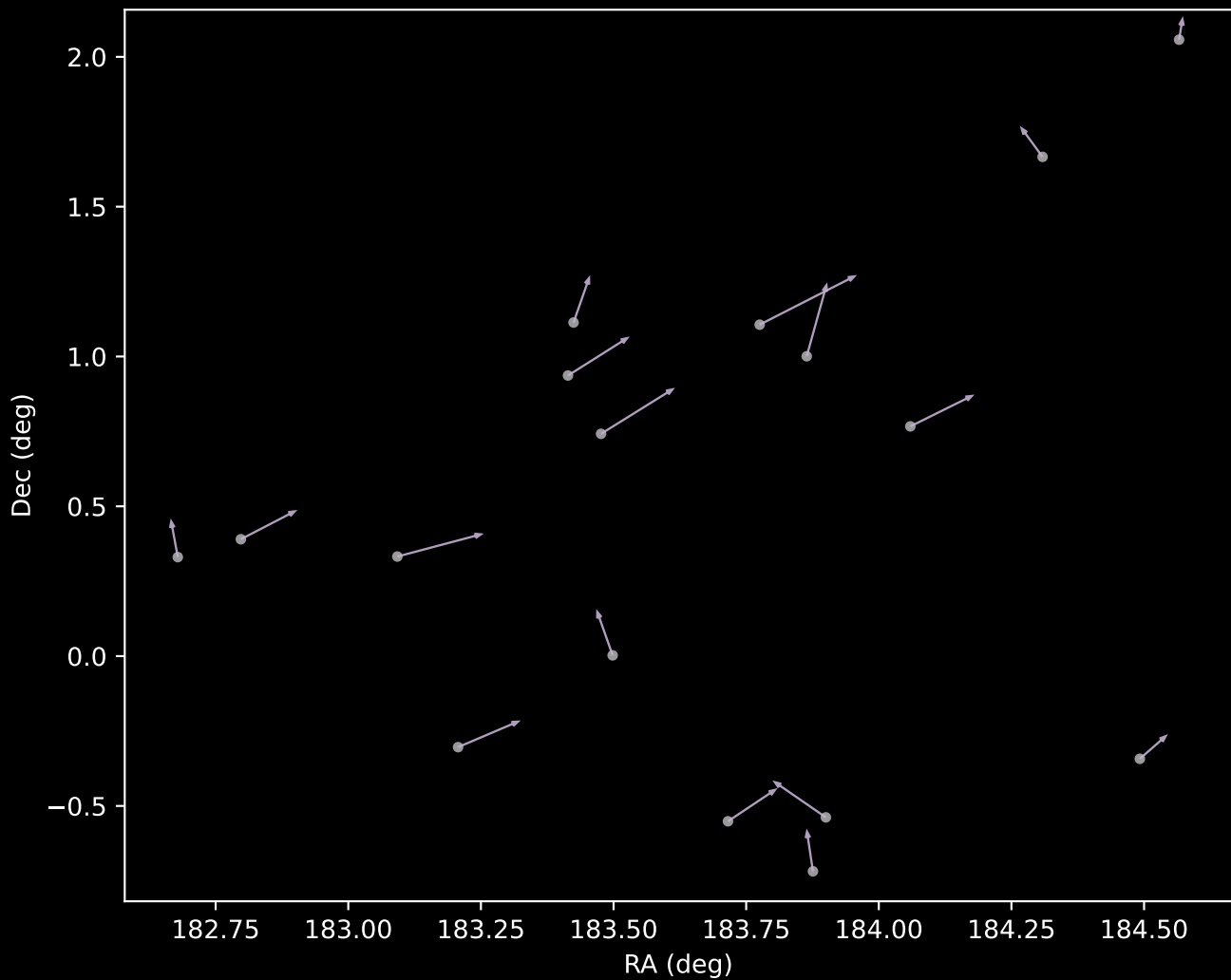
APOGEE DR17 Cluster 9 Proper Motion Vectors (n=17)
