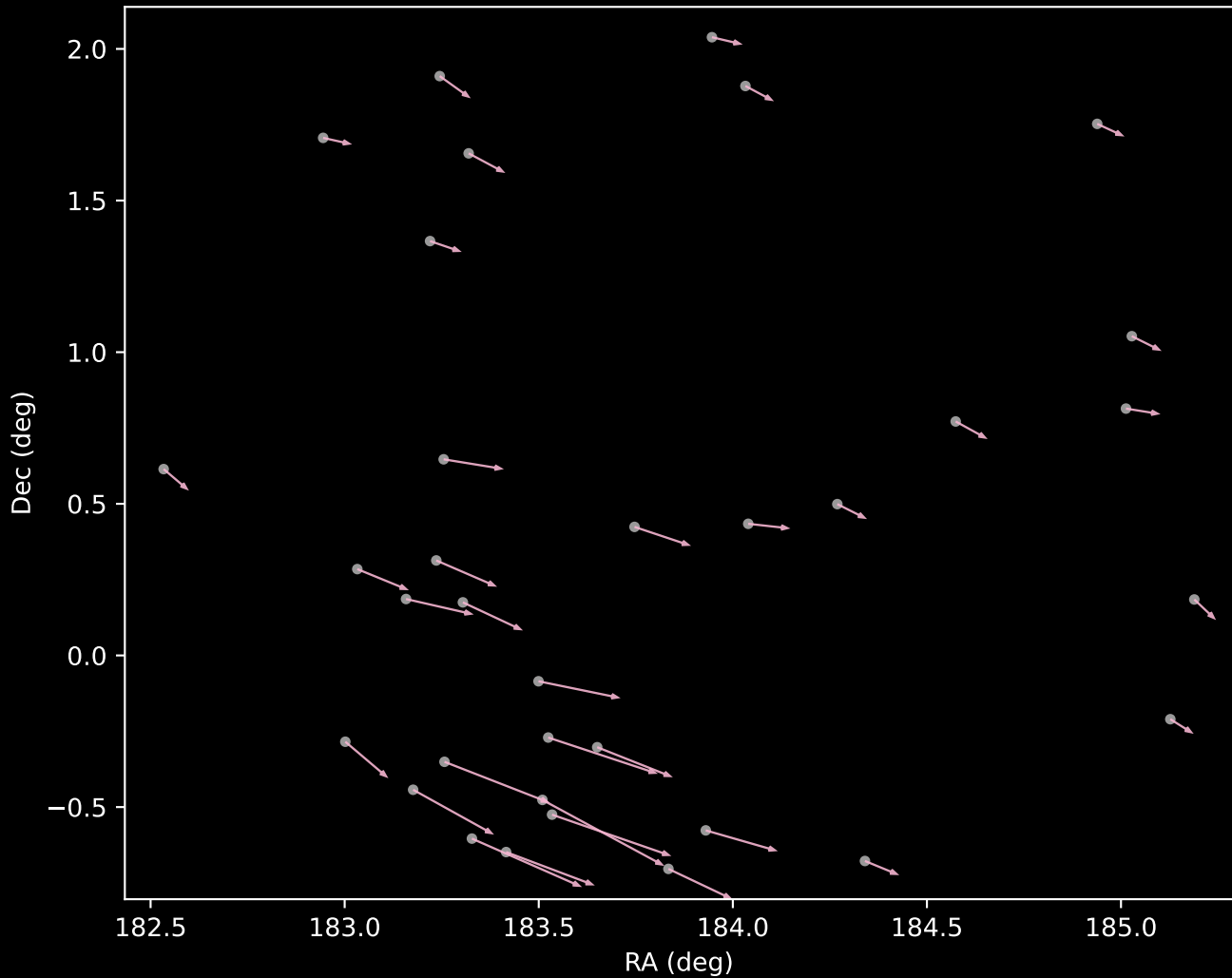
APOGEE DR17 Cluster 13 Proper Motion Vectors (n=34)
