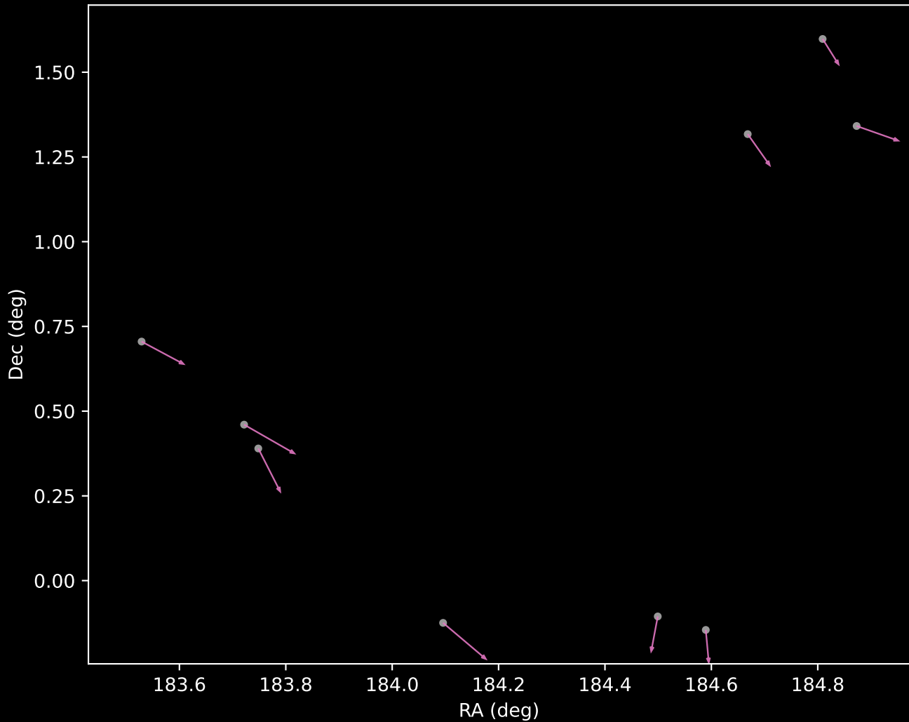
APOGEE DR17 Cluster 12 Proper Motion Vectors (n=9)
