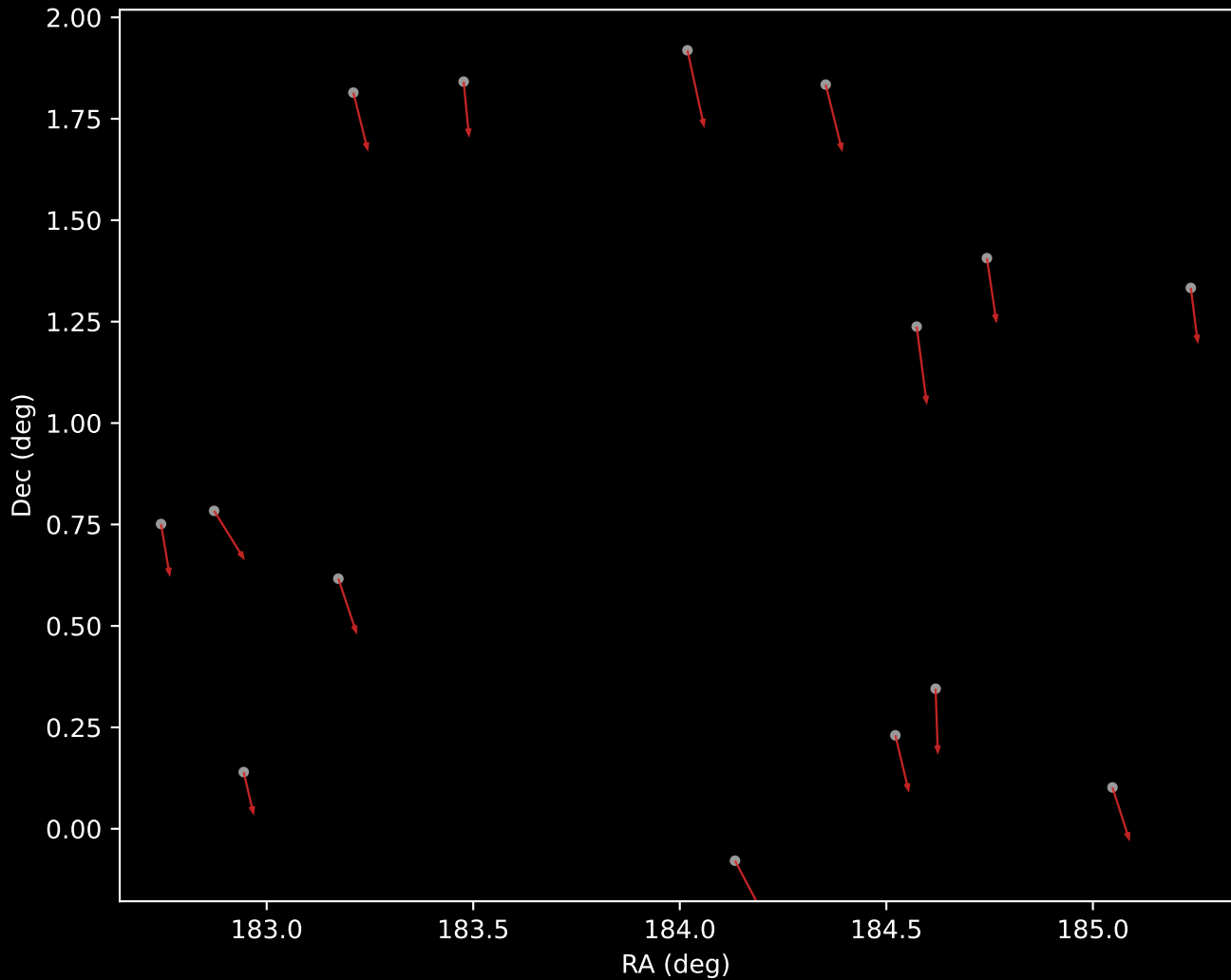
APOGEE DR17 Cluster 6 Proper Motion Vectors (n=15)
