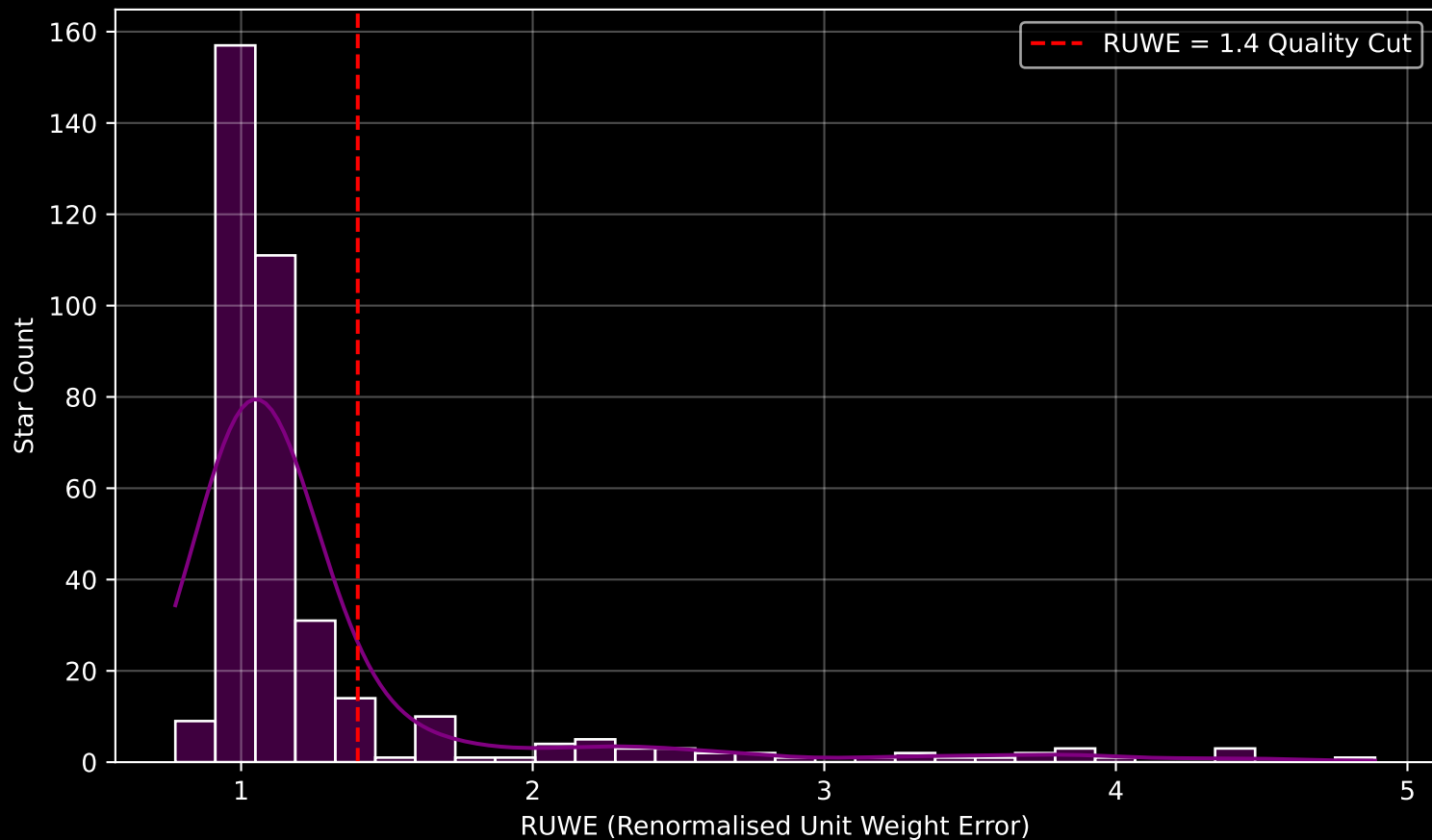
GAPOGEE DR17 Field [ORIONOB1AB-B] RUWE Distribution (n= 370)
